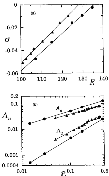
FIG. 3. (a) Growth rates \sigma below transition and (b) saturation amplitudes of the first two Fourier components, A_0 and A_1 , above transition are compared for u from the experiment at x=3.9 downstream of cylinder number 18, y=0 , and z=-5.1 ( \Delta ) and for v from the simulation (streamwise-periodic boundary conditions) at x=1.6666 and y=-0.5 ( \bullet ).
