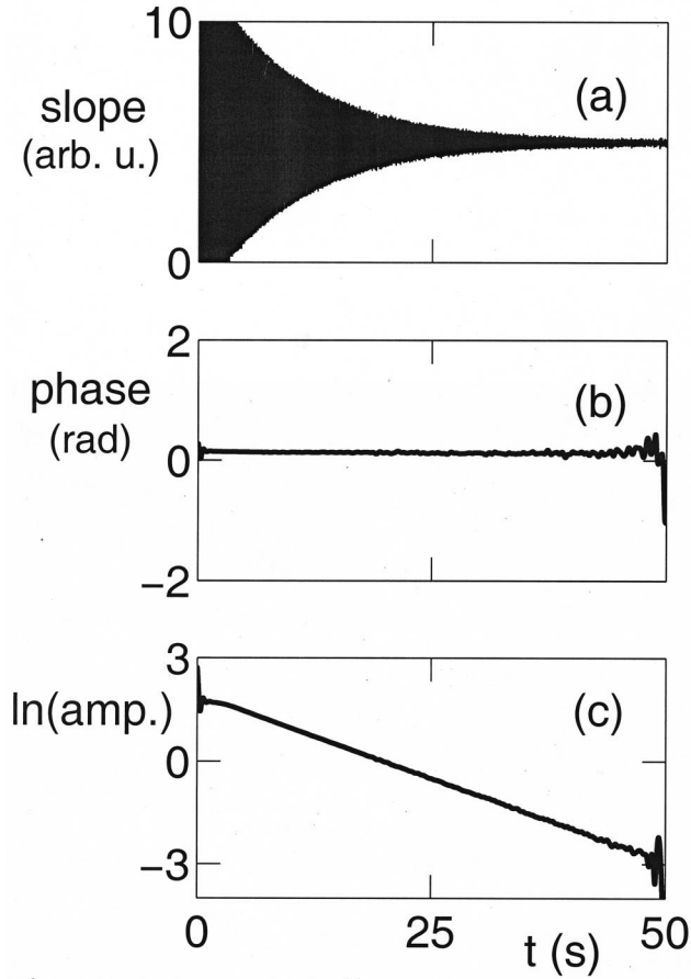
FIG. 2. Measured surface-slope time series (a), with complex-demodulated phase (b), and amplitude (c), for a (0,1) mode in silicone oil with C = 7.647 \times 10^{-5} and \Gamma = 0.725 .
