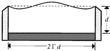
FIG. 1. Surface-wave damping is investigated in clean liquid layers with a contact line pinned to a circular lateral boundary, as shown in a schematic cross section of the experiment. The experimental conditions are described by the aspect ratio \Gamma , the inverse Reynolds number C \equiv (\nu/\sqrt{g(d\Gamma)^3}) and the Bond number B \equiv g\rho(d\Gamma)^2/\sigma with the liquid's depth d , density \rho , surface tension \sigma , kinematic viscosity \nu and the earth's gravitational acceleration g .
