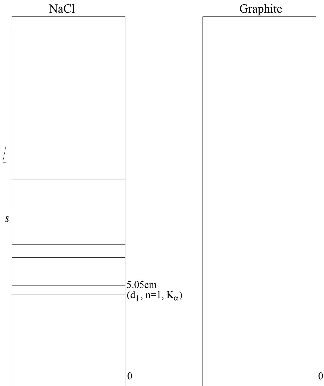
Figure 7: Copy of powder diffraction film from NaCl (left) The zero corresponds to the straight through beam (i.e., 2\theta = 0 ). The right side is a blank film strip for a graphite diffraction pattern
